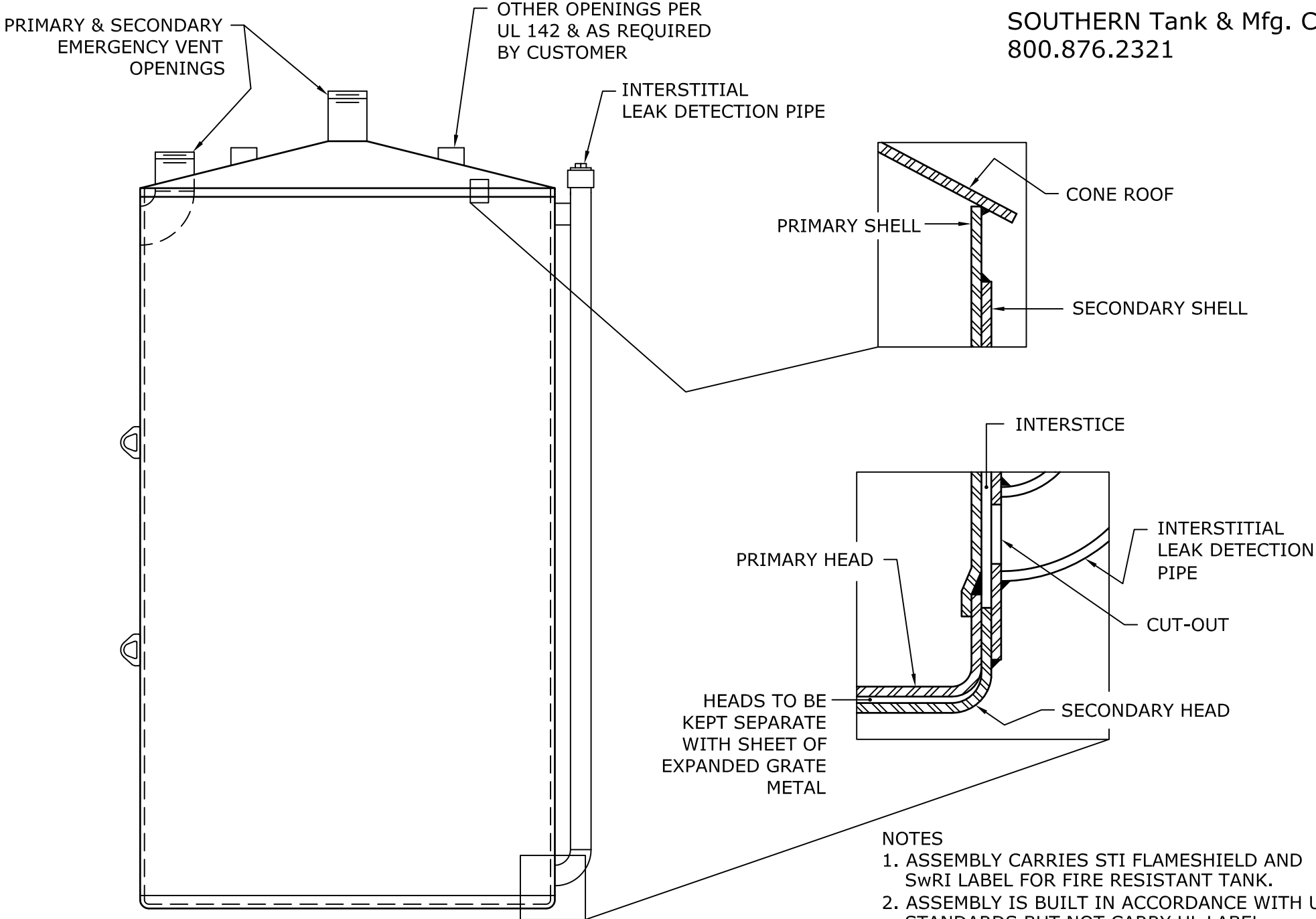
TANK DIAGRAM: FLAMESHIELD VERTICAL
